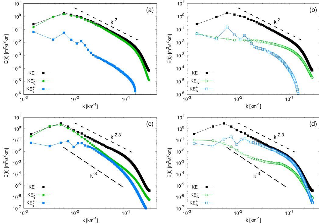
FIG. 11. Wavenumber spectra of kinetic energy E(k) in the Kuroshio Extension region. The spectrum of the total KE is shown by black square points. (a),(c) Spectra of the rotational component KE_{\zeta}^{-} ; (b),(d) spectra of the divergent component KE_{\Delta}^{+} . In each case, the flow is further partitioned into low- and high-frequency motions as in Fig. 10. (a),(b) February; (c),(d) August.
